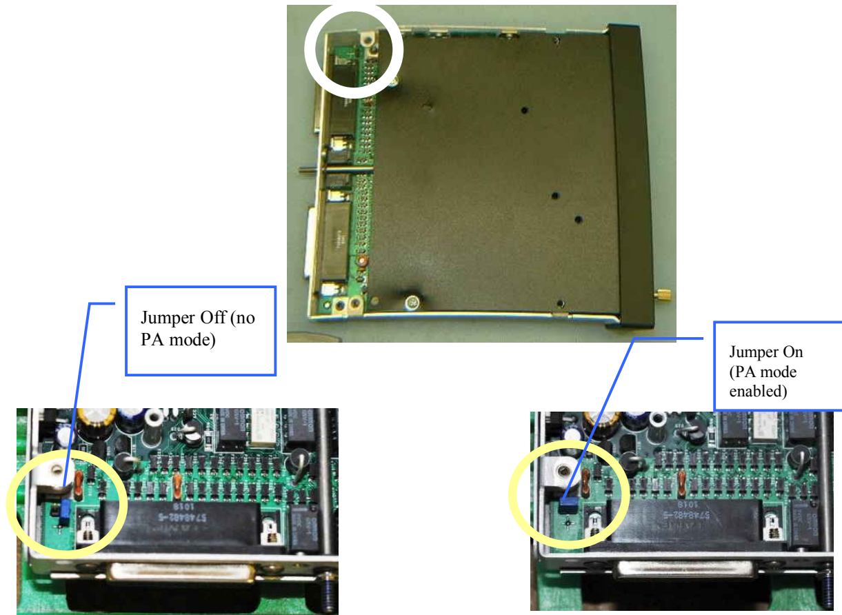
Figure 2-3 Jumper Location
