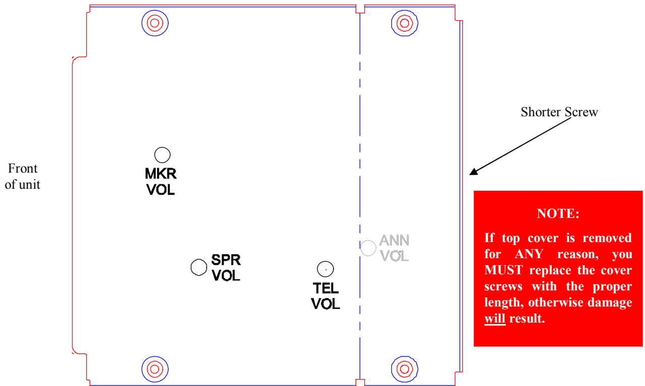
Figure 2-4- PMA8000B-MP3 Adjustments, top cover
