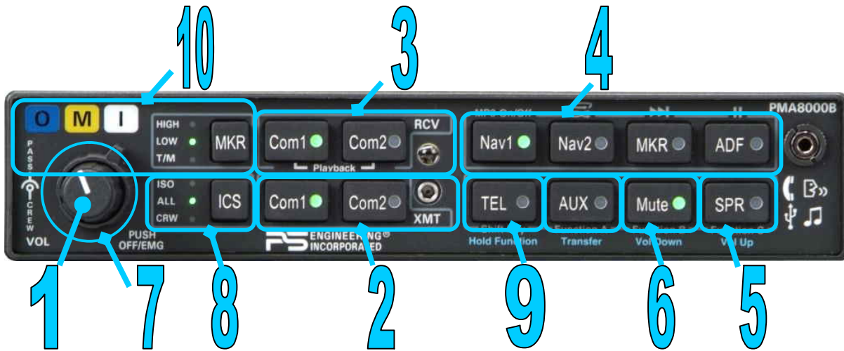
Figure 3-1 PMA8000B-MP3 Operating controls
