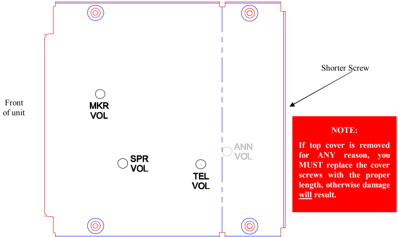
Figure 2-2- PMA8000B-MP3 Adjustments, top cover
